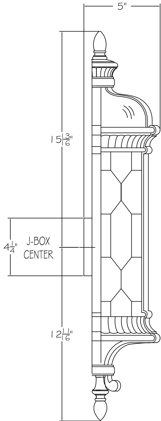
SIDE VIEW
